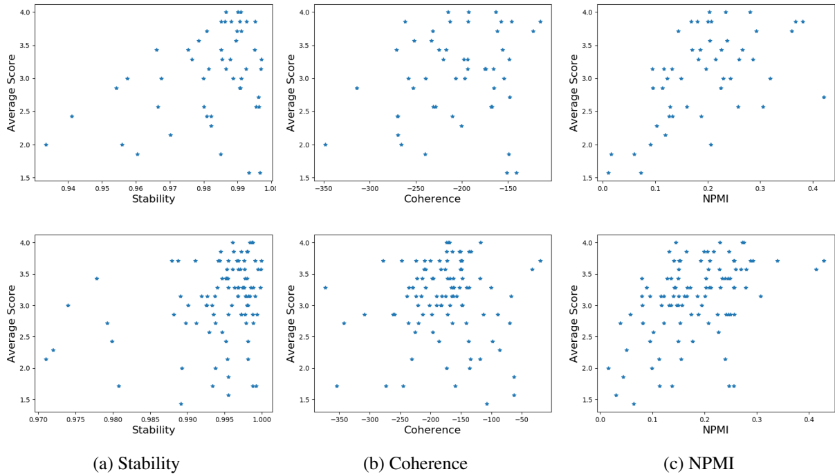
Figure 1: Human-provided topic ratings along with stability, coherence and NPMI scores for the News (top, 50 topics) and Wiki (bottom, 100 topics) datasets.
