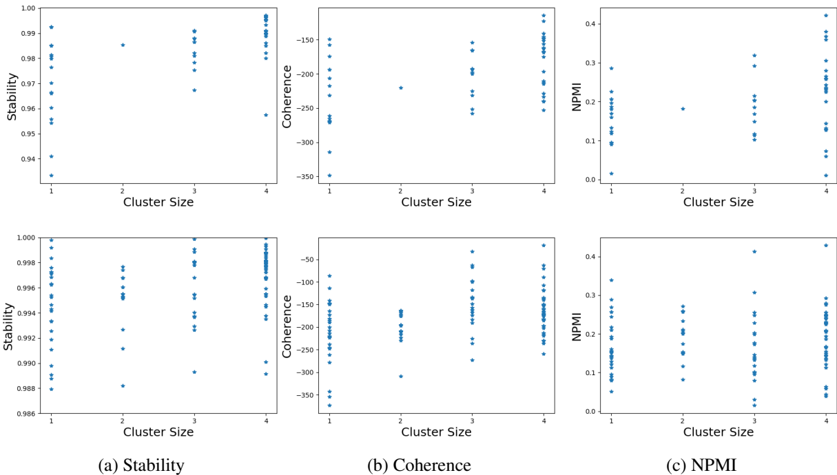
Figure 2: Distribution of topic stability, coherence and NPMI scores within different sized clusters on the topic alignment task for the News (top) and Wiki (bottom) datasets. The topics in larger cluster sizes indicate they are easier to be replicated across multiple runs of LDA. On both datasets, topic stability is aligned relatively well with the cluster size. The number of topics within each cluster size (1, 2, 3, and 4, respectively) are 16, 1, 11, and 22 on News and 26, 15, 20, and 39 on Wiki .
